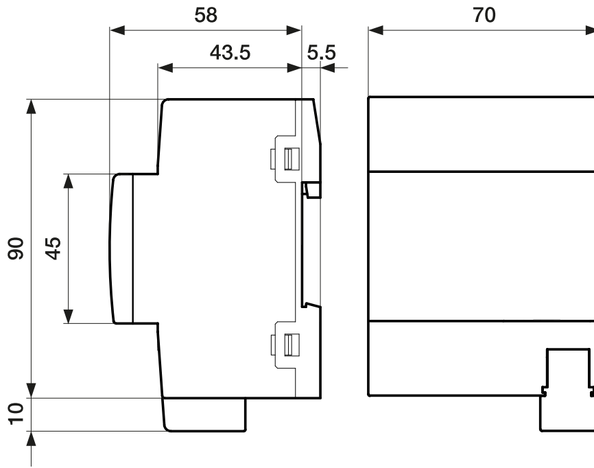
Fig. 11: Dimension drawing
