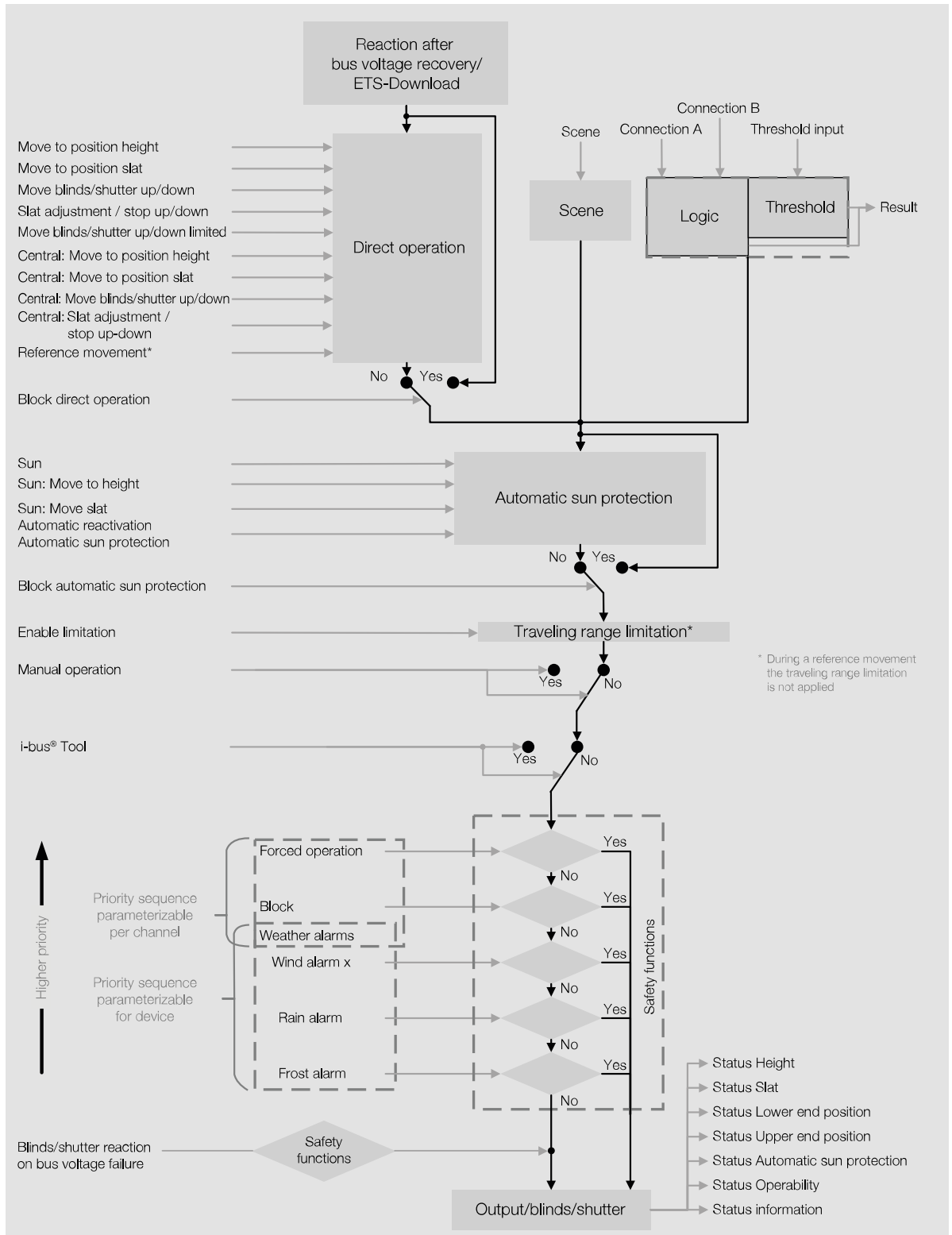
Fig. 28: Function diagram Shutter Actuator
