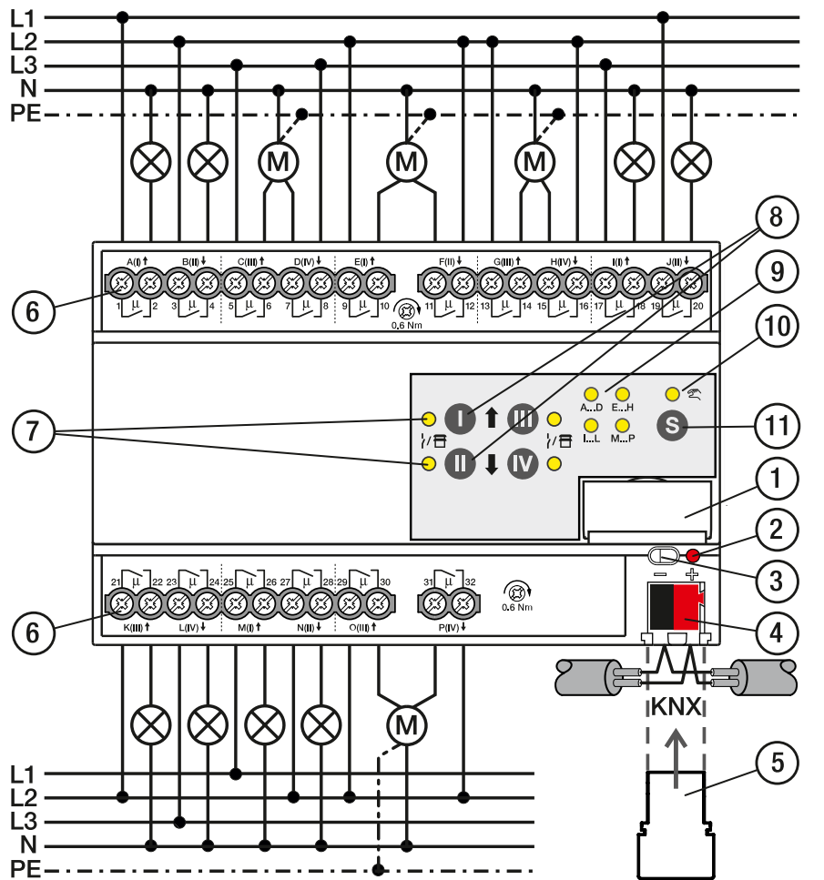
Fig. 24: Connection diagram SAH/S 16.x.7.1
