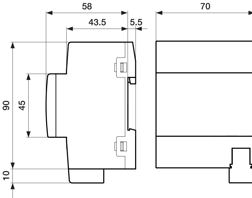
Fig. 20: Dimension drawing
